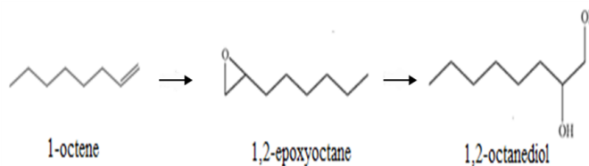
Figure 1. Formation of 1,2-octanediol from 1-octene Through 1,2-epoxyoctane Generation
