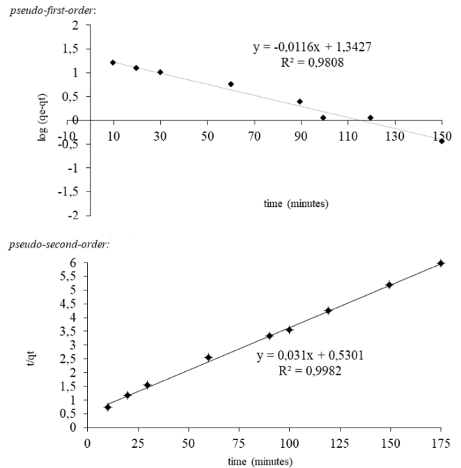
Figure 1. First-order kinetic modeling and Second-order kinetic modelling of adsorption of Cr(VI) onto dried Oscillatoria Splendida
